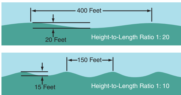
Figure 8-2. Height-to-length ratio.
