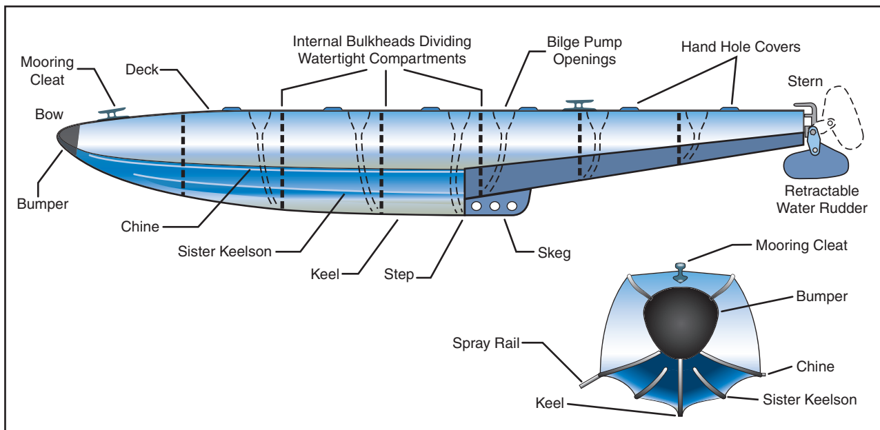
Figure 2-3. Float components.
